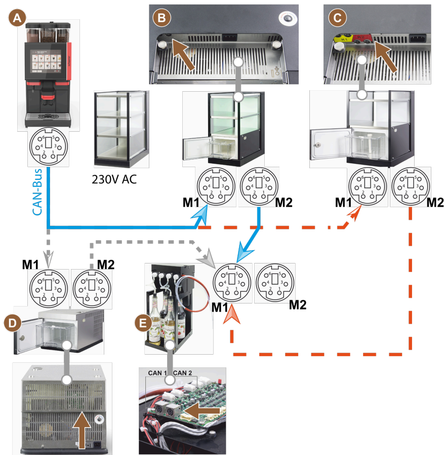
Figure: CAN bus connections from the machine to optional accessories (example display)
