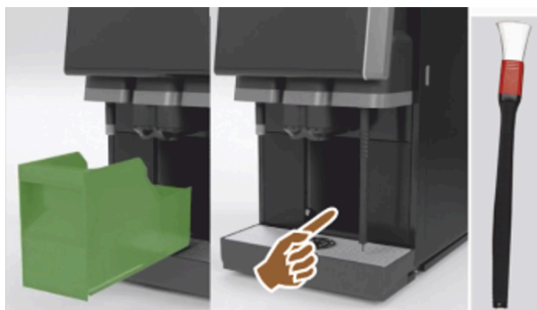
Figure: Cleaning brewing chamber
