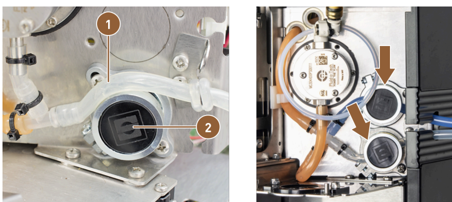
Figure: Inserting milk hoses into squeeze valves (Twin Milk)
