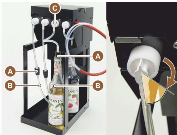
Figure: Flavour Point: Refill or bottle change
