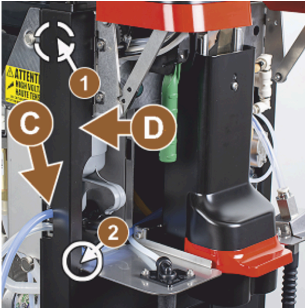
Figure: Milk hoses through side strip
