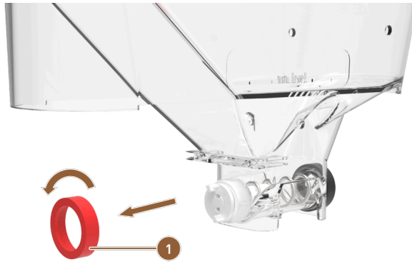
Figure: Standard powder container: Removing cap nut on feed side
