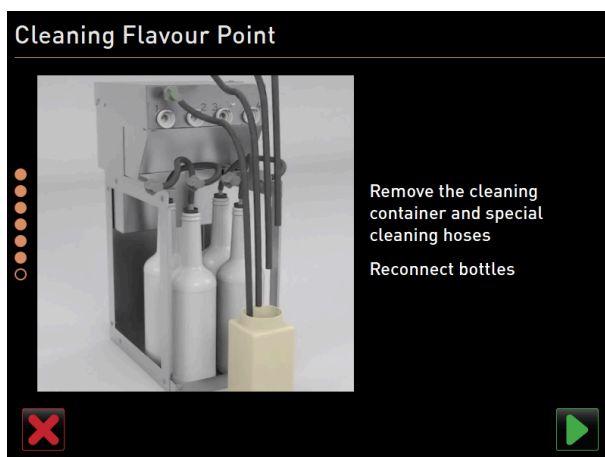
Figure: Removing cleaning container
