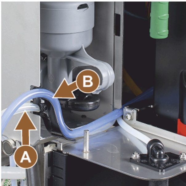
Figure: Milk hose in guide
