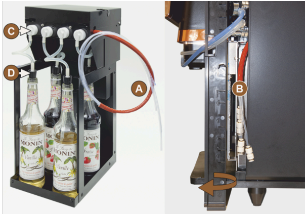
Figure: Flavour Point SOUL hose connection
