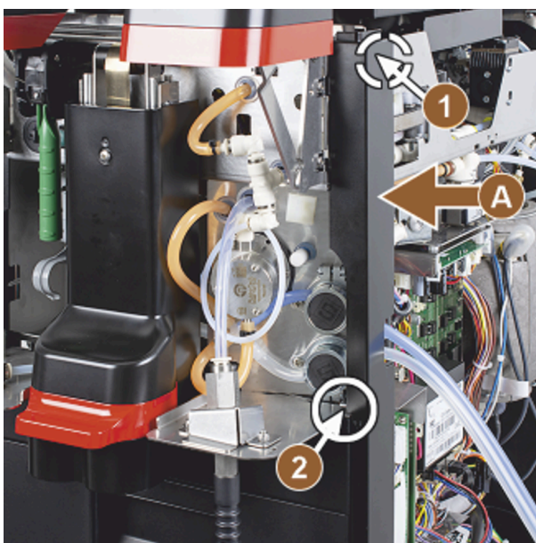
Figure: Side strip fastening
