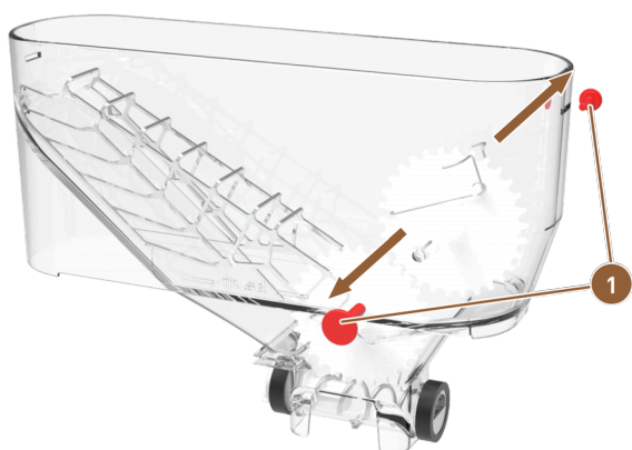
Figure: Standard powder container: Removing locking pin
