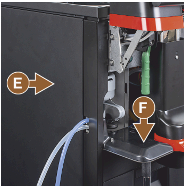
Figure: Assembling side housing
