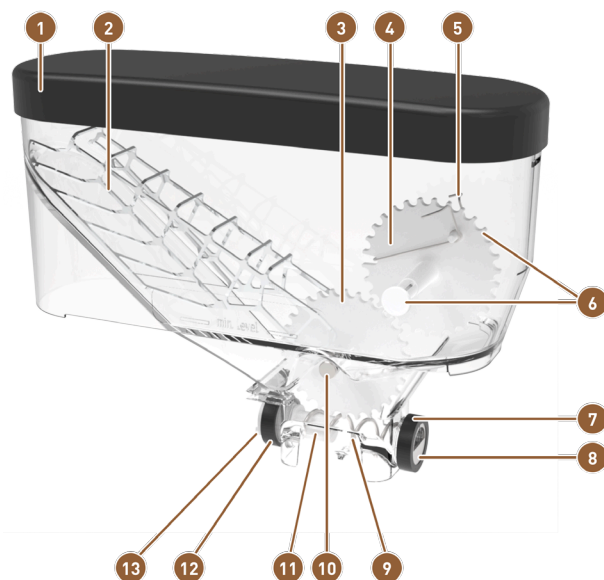
Figure: Parts of the standard powder container (2 kg)
