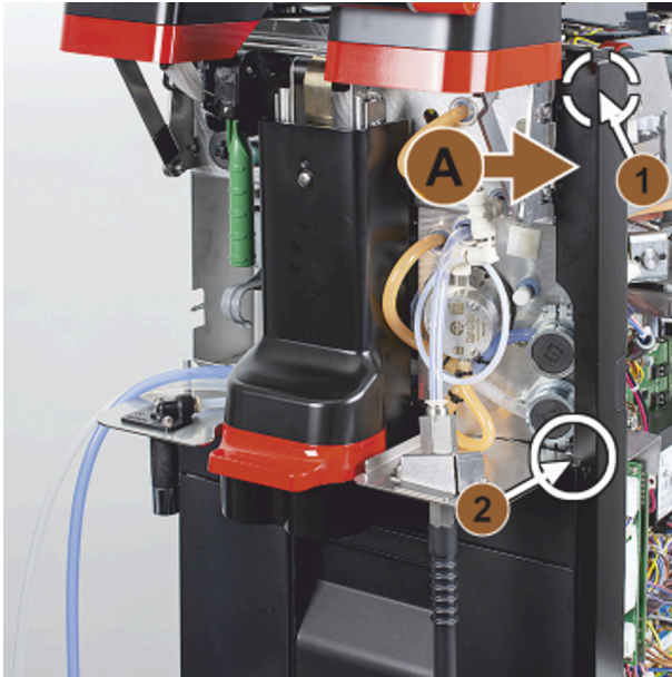
Figure: Assembly of the right side strip
