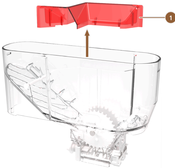
Figure: Twin powder container
