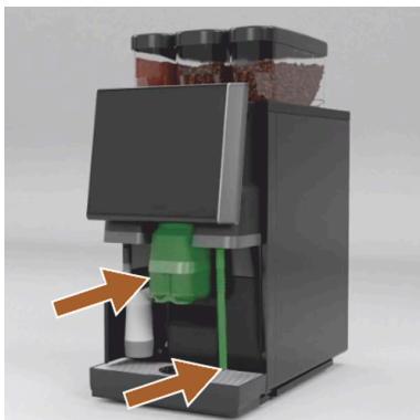
Figure: Removing cup platform
