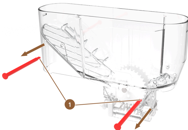
Figure: Twin powder container: Removing crossbars
