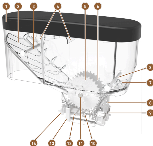
Figure: Parts of the Twin powder container (2x 1 kg)
