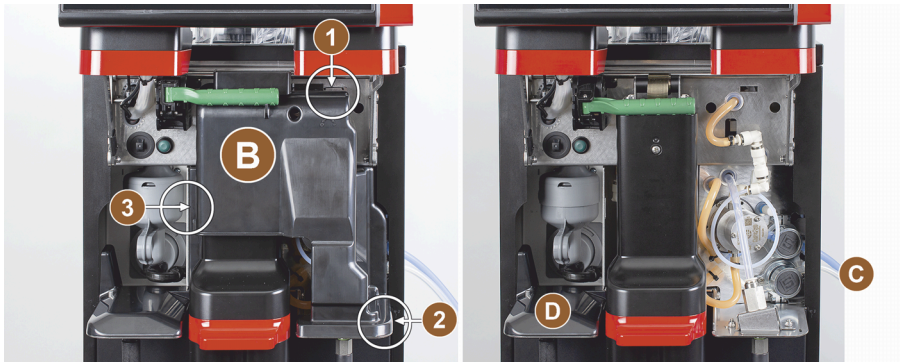
Figure: Removing squeeze valve cover
