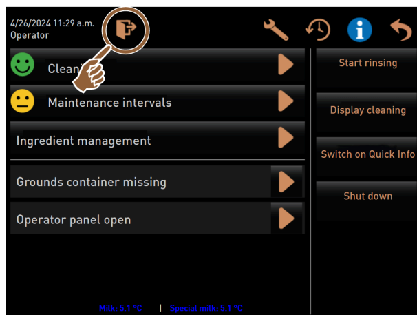
Figure: Log-in/Log-out
