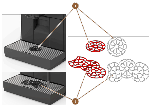
Figure: Cup positioning aid
