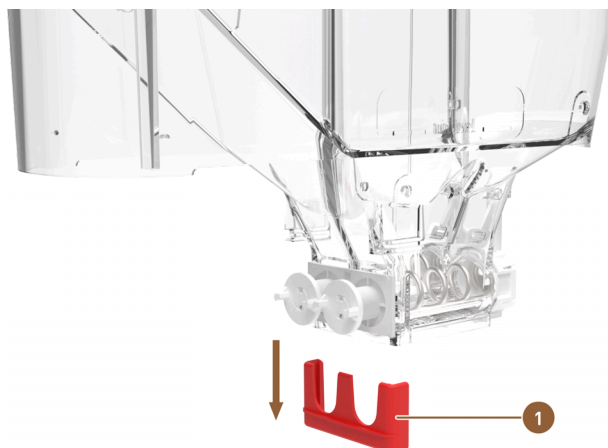
Figure: Twin powder container: Removing drive holder
