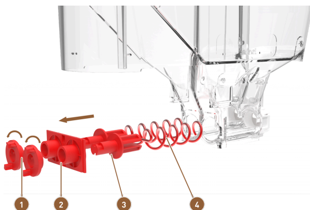
Figure: Twin powder container: Disassembling supply unit
