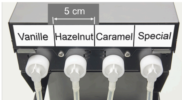
Figure: Labelling example for hose connections from syrup bottle to syrup pump
